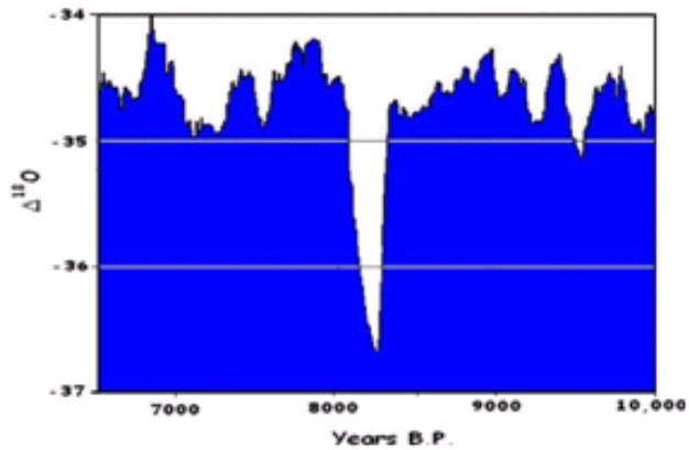
Figure 5.12.2. The 8,200 y BP sudden cooling recorded in oxygen isotope ratios in the GISP2 ice core. Adapted from Easterbrook, D.J. (Ed.) 2011. Evidence-based climate science: Data opposing CO 2 emissions as the primary source of global warming. Elsevier.
