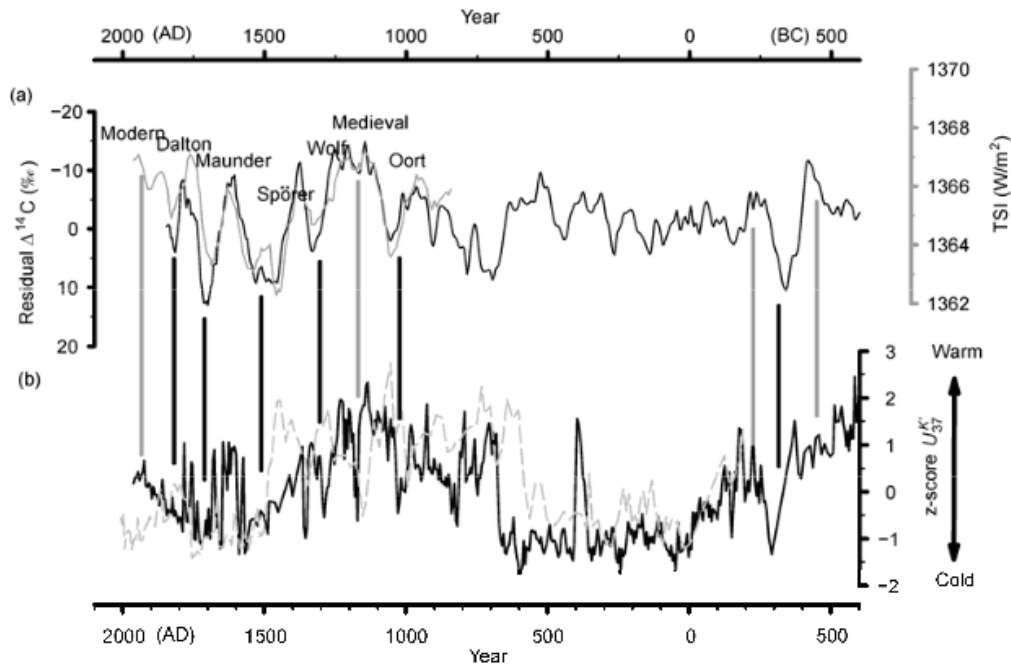
Figure 3.3.5.1. Correlations between solar activity proxies (top curves: TSI-grey; ^{14}\text{C} -black) and temperature proxies (bottom curves: Lake Sungan-grey; Lake Gahai-black) from northern Tibetan Plateau. Reprinted with permission from He, Y.X., Liu, W.G., Zhao, C., Wang, Z., Wang, H.Y., Liu, Y., Qin, X.Y., Hu, Q.H., An, Z.S., and Liu, Z.H. 2013. Solar influenced late Holocene temperature changes on the northern Tibetan Plateau. Chinese Science Bulletin 58 : 1053–1059.
